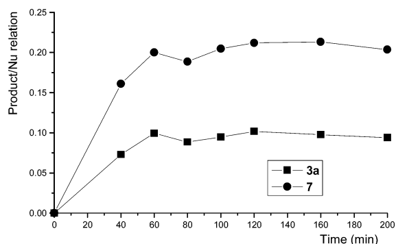
FIGURE 1. Product relationship obtained by sampling the reaction of 1 with o -bromiodobenzene at different irradiation times: (■) 3a ; (●) 7 .
